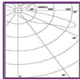
TIPO III Non-Cutoff
